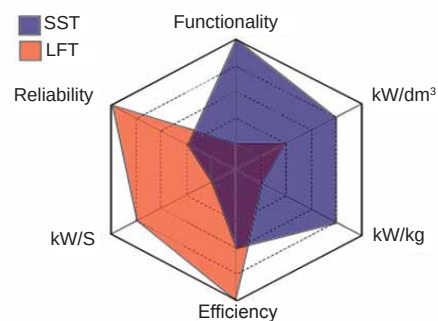
Figure 2.6: Comparison between LFT and SST[6]
